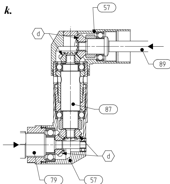
(remontage M180)
